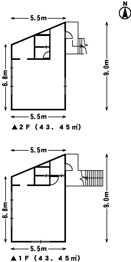
[間取り図]
